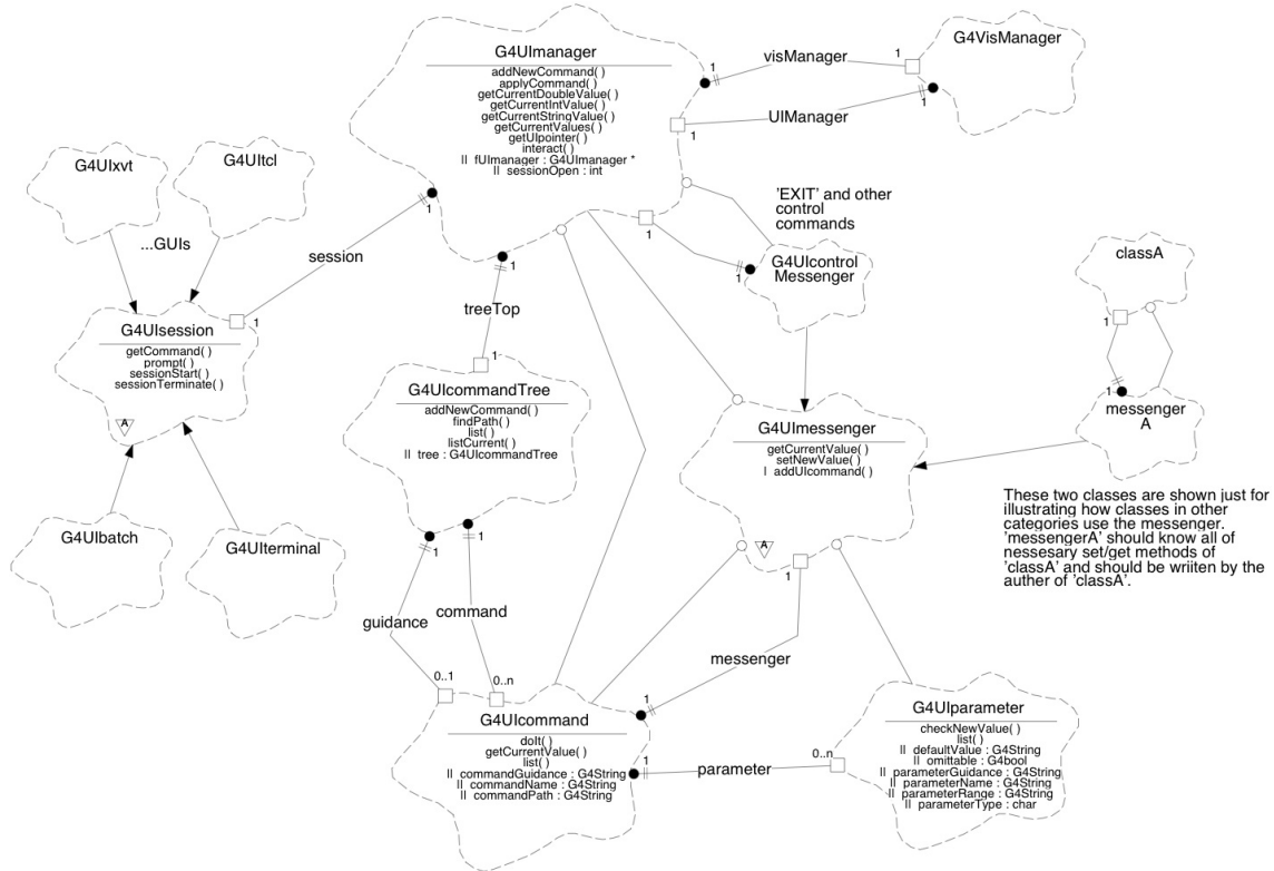
Fig. 2.25: Overview of intercom classes
