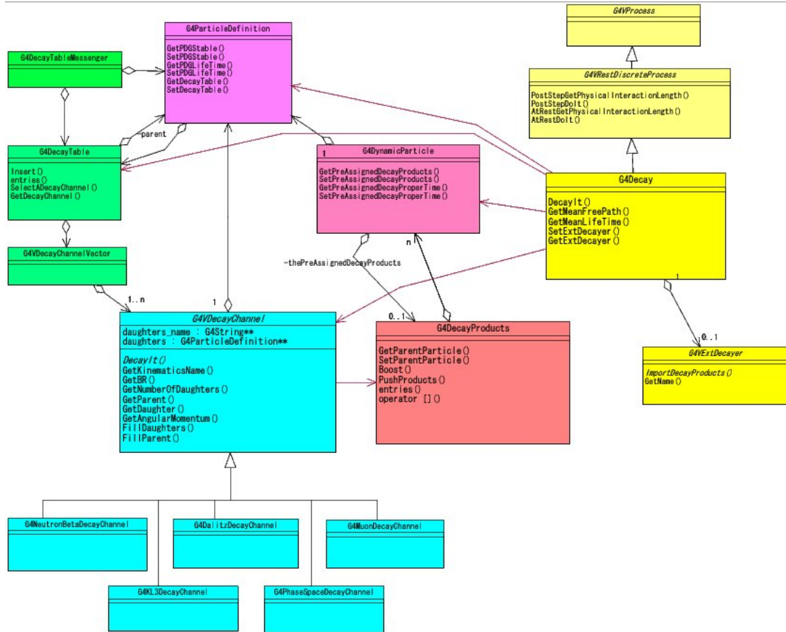
Fig. 2.21: Particle Decay
