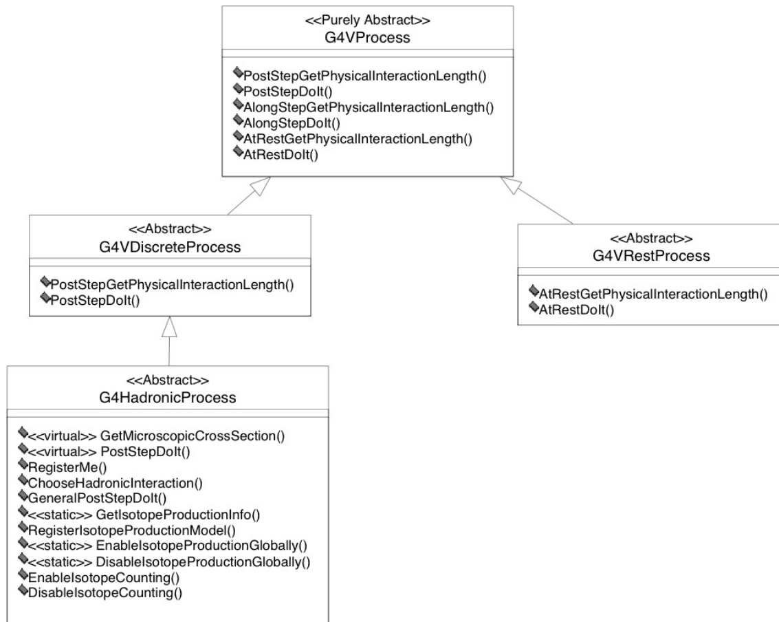
Fig. 2.9: First level implementation framework of the hadronic category of GEANT4.
