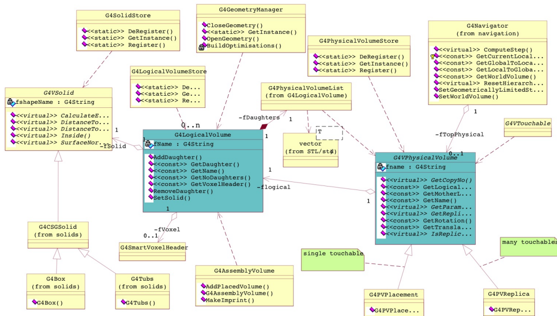
Fig. 2.13: Overview of the geometry.
