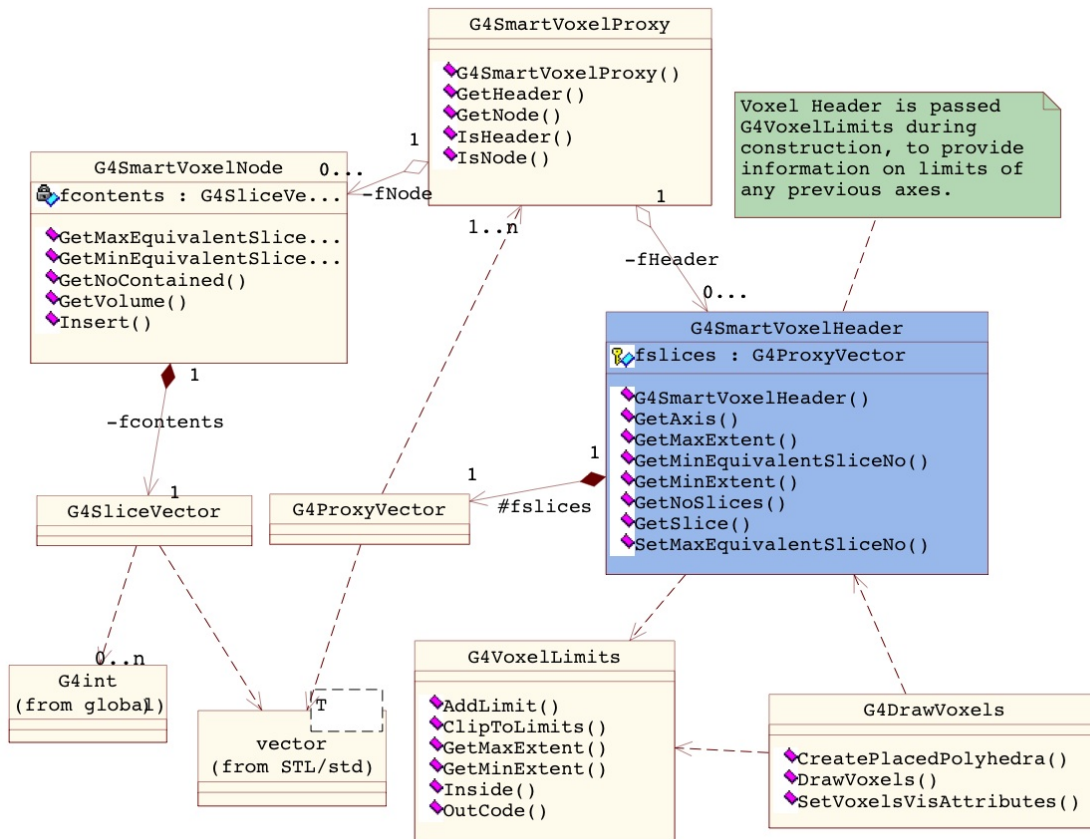
Fig. 2.14: Class diagram for smart voxels
